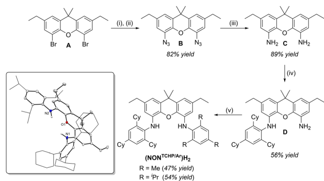
Scheme 1 Synthesis of unsymmetrical bis(anilino)xanthene pro-ligands. (i) n BuLi (2 equiv.), THF, -78\text{ }^{\circ}\text{C} . (ii) Tosylazide (2 equiv.), THF, -78\text{ }^{\circ}\text{C} – RT, 18 h. (iii) \text{LiAlH}_4 (3 equiv.), \text{Et}_2\text{O} , reflux, 2 h. (iv) (TCHP)Br (1 equiv.), \text{Pd}(\text{OAc})_2 (4 mol%), DPEPhos (6 mol%), \text{NaO}^t\text{Bu} (1.4 equiv.). (v) (Mes)Br (1 equiv.) or (Trip)Br (1 equiv.), \text{Pd}(\text{OAc})_2 (4 mol%), DPEPhos (6 mol%), \text{NaO}^t\text{Bu} (1.4 equiv.). Inset: Molecular structure of (\text{NON}^{\text{TCHP/Trip}})^-\text{H}_2 . Thermal ellipsoids shown at 15% probability; hydrogen atoms (except amine protons) omitted; cyclohexyl and isopropyl groups shown in wireframe for clarity.
