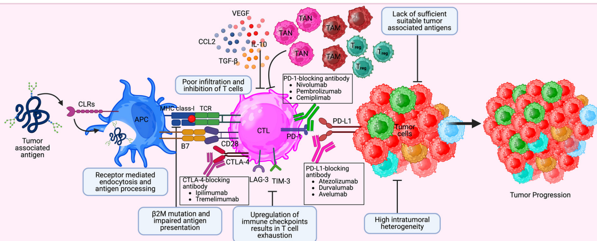
Fig. 2 Response and resistance to ICIs: (a) a successful anti-tumor immune response following ICIs requires reactivation and proliferation of T cells. Production of tumor-reactive CD8 + T cells requires successful tumor-associated peptide antigen processing and presentation by the APCs. TCRs recognize the tumor antigens that are presented by the MHC, providing a signal for T cell activation. This activation additionally necessitates the interaction of the co-stimulatory CD28 receptor expressed on T cells with B7 present on the APCs. Tumor-specific CD8 + T cells then further differentiate into effector T cells and lead to tumor cell apoptosis through release of granzyme A/B and perforin and decrease the immunosuppressive capacity of the TME; (b) resistance to ICIs originates when the various stages of the cancer immune cycle are disrupted or blocked. In immunosuppressive TMEs, factors such as inefficient antigen presentation, poor infiltration and suppressed activity of CD8 + T cells, and failure of antigen recognition can reduce antitumor immunity. Loss of sufficient neoantigens and their impaired presentation can lead to decreased T cell cytotoxicity. High intratumor heterogeneity can also result in an ineffective recognition of tumor-specific neoantigens and reduced CTL responses. In addition, mutations in the antigen processing and presentation machinery can trigger resistance to ICIs. The loss of \beta 2M expression leads to a decline in MHC class I cell surface expression, which impairs the antigen presentation to CTLs. Immune cells within the TME, such as T cells, neutrophils, and M \phi s, are reprogrammed to become pro-tumor cells, which prevent T cells from functioning by activating various ICs and secreting cytokines, including IL-10, VEGF, CCL2, and TGF- \beta (created in BioRender. Jain, M. (2025) https://BioRender.com/j05c775 ).
