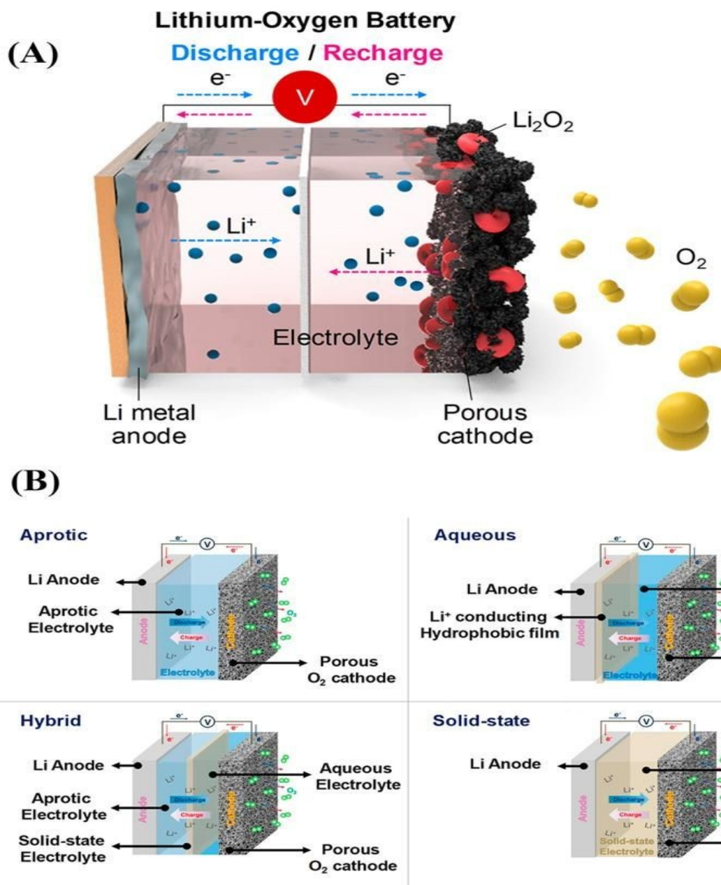
Fig. 9 (A) Schematic presentation of Li-O 2 battery. (B) Schematic configuration of all types of Li-O 2 cells [145].
