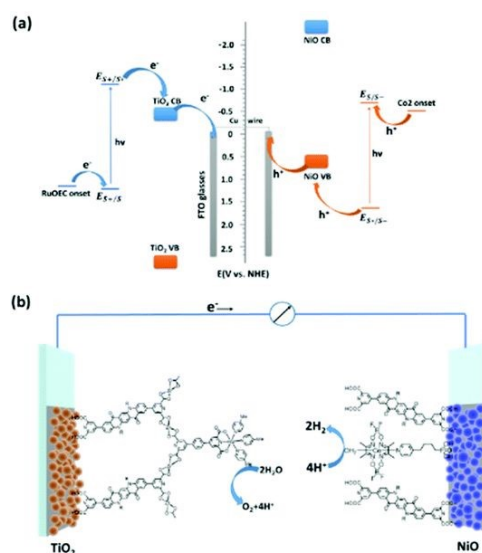
Figure 11. QA based photoelectrochemical cell for water splitting into hydrogen and oxygen: representation of the energy levels (a) and molecular assembly of the cell (b). Reproduced from ref. 58 with permission from the Royal Society of Chemistry, copyright 2022.
