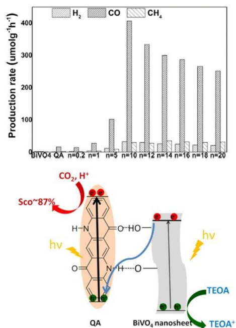
Figure 8. Top panel: Production rates from \text{CO}_2 photoreduction (average over 10 h) on \text{BiVO}_4 , QA, and \text{QA}/n\text{BiVO}_4 for 10 h. n is the mass ratio between \text{BiVO}_4 and QA, impacting the photocatalytic performance. Bottom panel: Schematic representation of photochemical \text{CO}_2 reduction on QA/ \text{BiVO}_4 composites. Reproduced from ref. 50 with permission from Wiley Inc., copyright 2020.
