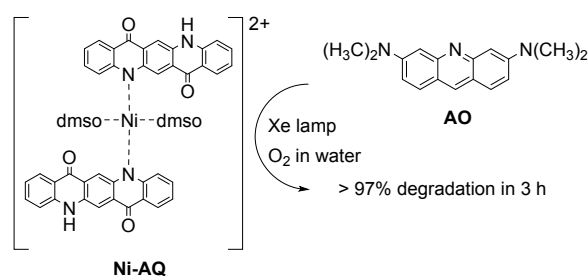
Figure 5. Ni-AQ complex (obtained as the nitrate salt) for the aerobic photodegradation of acridine orange (AO) in water with visible light. 44
