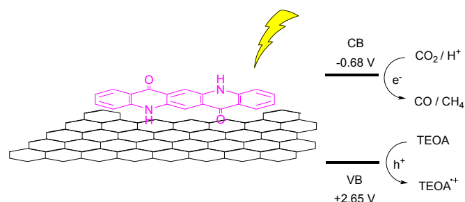
Figure 7. Reduction of CO 2 over QA/rGO photocatalyst, and schematic representation of CO 2 reduction to CO and CH 4 , coupled with oxidation of triethanolamine (TEOA); the potential of the conduction and valence bands (CB and VB, respectively) are reported versus the reversible hydrogen electrode. 49
