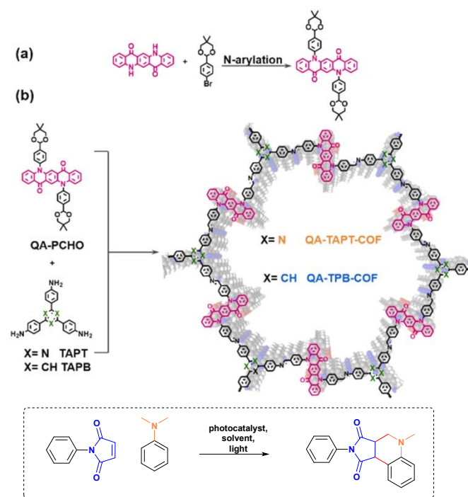
Figure 9. Incorporation of QA derivatives in 2D covalent organic frameworks and photochemical application towards the Povarov reaction. Reproduced from ref. 53 with permission from Elsevier, copyright 2022.
