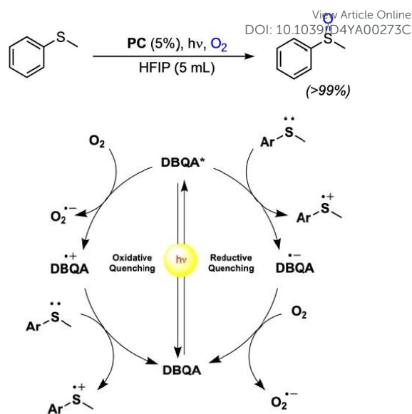
Figure 4. Photocatalytic oxidation of thioethers with QA derivatives, and proposed reaction mechanism on the basis of scavenging experiments. Reproduced from ref. 43 with permission from Wiley Inc., copyright 2023.
