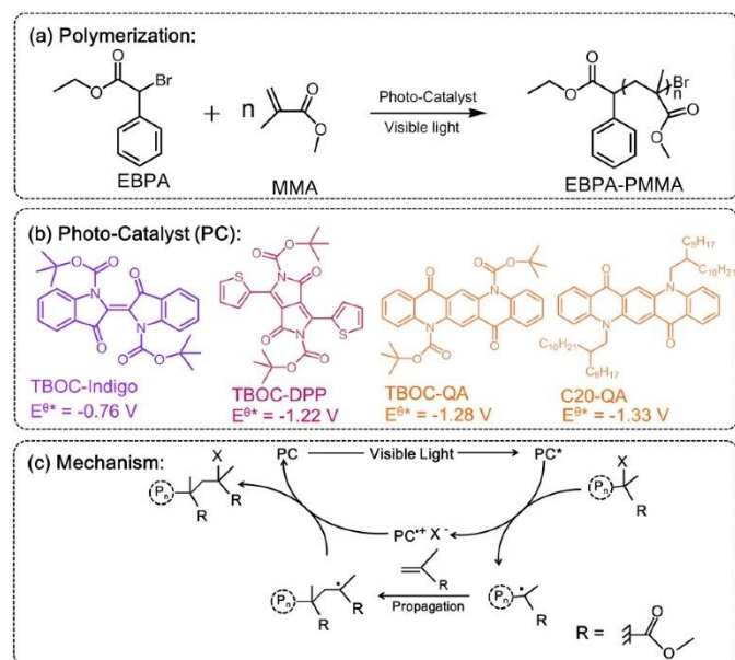
Figure 3. QA based derivatives employed for photocatalysed polymerization reaction of MMA, and proposed mechanism (Adapted from ref. 34 with permission from Elsevier, copyright 2019)
