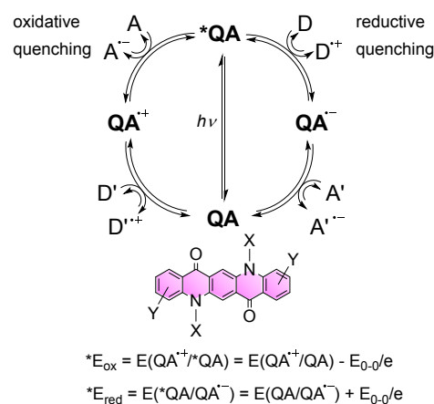
Scheme 3. Representation of possible reaction pathways of the *QA excited state through oxidative and reductive quenching, leading to the generation of oxidised QA + and reduced QA - , respectively. A and A' represent electron acceptors, while D and D' represent electron donors. The two equations enable the estimation of *E ox and *E red of the *QA excited state. 41,42
