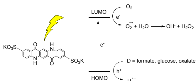
Figure 6. Water soluble QA disulfonate derivative, and photochemical hydrogen peroxide production coupled to oxidation of donors D. Adapted from ref. 46 with permission from Wiley Inc., copyright 2019.
