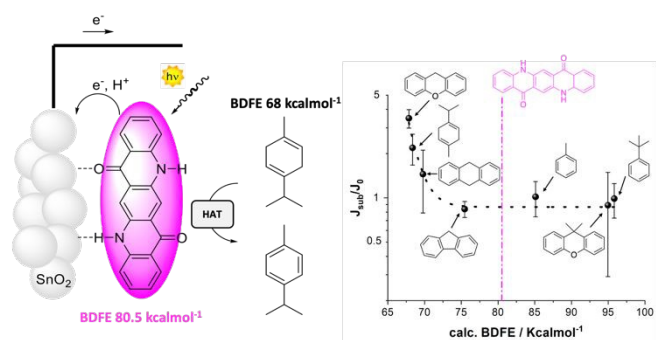
Figure 13. QA based photoanode for oxidative C-H activation. The right figure shows the photoelectrochemical response (given by the ratio of the photocurrent in the presence and in the absence of the organic substrate) versus the BDFE of the C-H bond of the substrate. Reproduced from ref. 31 with permission from Wiley Inc., copyright 2023.
