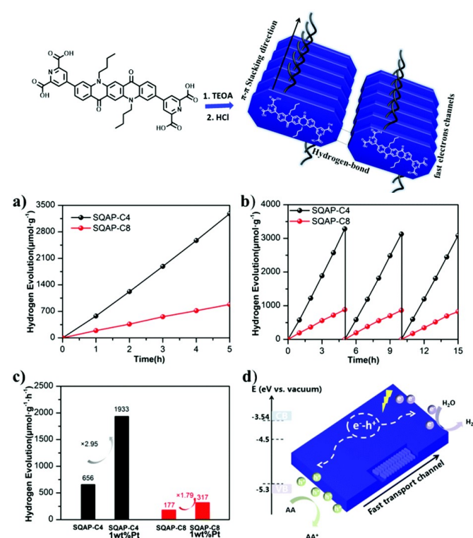
Figure 10. Formation of QA based nanobelts, and application in photocatalytic water reduction to hydrogen. Reproduced from ref. 54 with permission from the Royal Society of Chemistry, copyright 2020.
