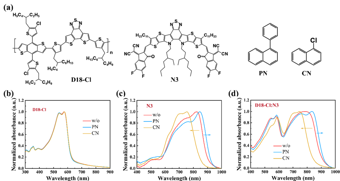
Fig. 1 (a) Chemical structures of D18-Cl, N3 and solvent additives PN and CN. (b)–(d) The absorbance of neat D18-Cl, neat N3 and D18-Cl:N3 blend films without and with different additives (0.5 vol%).
