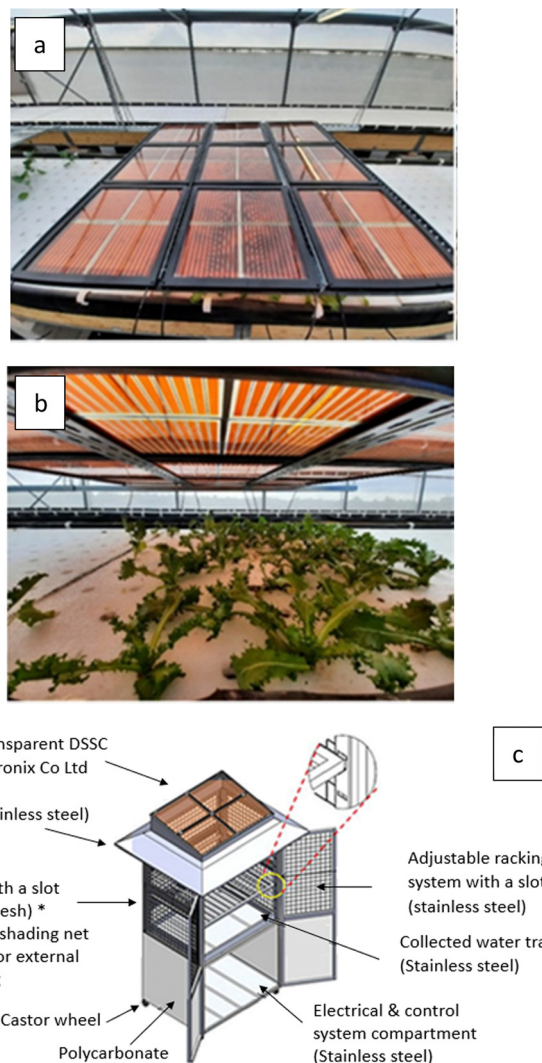
Fig. 12 (a) and (b) DSSM application in an Aquaponic greenhouse. 17 (c) The detailed construction drawings of PDMG prototype. Reproduced with permission ref. 233 Elsevier.
