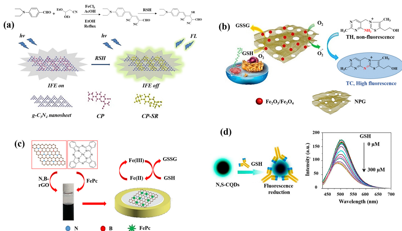
Fig. 2 Schematic illustration of GSH detection with carbon-based nanomaterials: (a) the IFE-based fluorescence sensor g-C_3N_4 nanosheets/CP, 42 (b) the MNPG-based fluorescent assay, 44 (c) the FePc/N,B-rGO nanocomposite, 46 and (d) graphical example of the N,S-CQDs fluorescence response to GSH along with the fluorescence spectra of N,S-CQDs combined with different levels GSH 47 reproduced with the permission of Elsevier and American Chemical Society.
