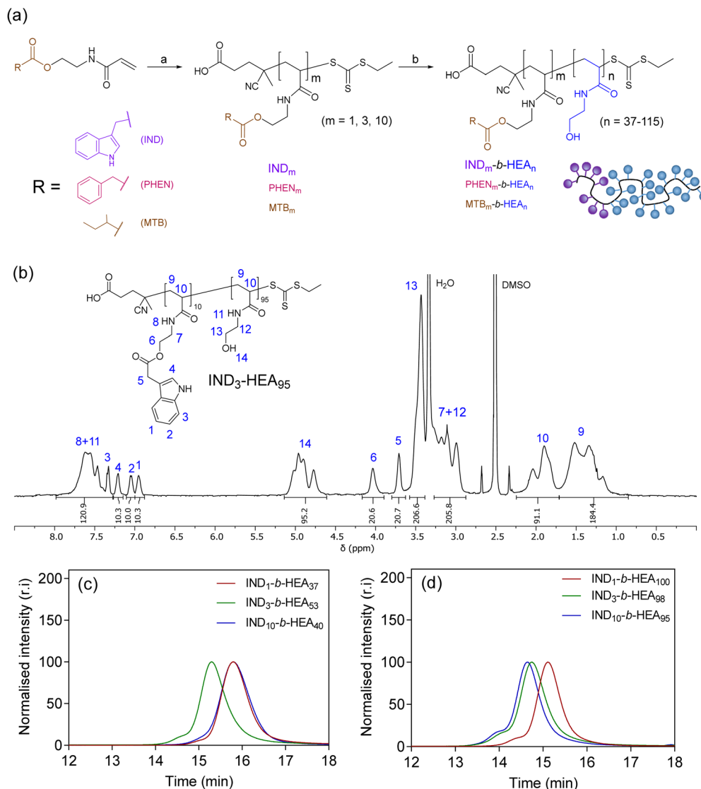
Fig. 3 (a) Synthesis of IND_m^- , PHEN_m^- , MTB_m^- - b - HEA_n block copolymers. Reagents and conditions: (a) AIBN, CTA, DMF, 80 °C; (b) N -hydroxyethyl acrylamide, V501, DMF, 70 °C; (b) ^1H NMR (DMSO- d_6 , 400 MHz) spectrum of IND_3 - HEA_{95} as a representative spectrum of the synthesised block copolymers; SEC chromatograms of IND_m^- - b - HEA_n copolymers with (c) shorter and (d) longer hydrophilic blocks, using DMF with 0.1% LiBr as the mobile phase. Spectra and SEC chromatograms of all polymers are shown in Sections S5.3.1 and S5.3.2 in the ESI.†
