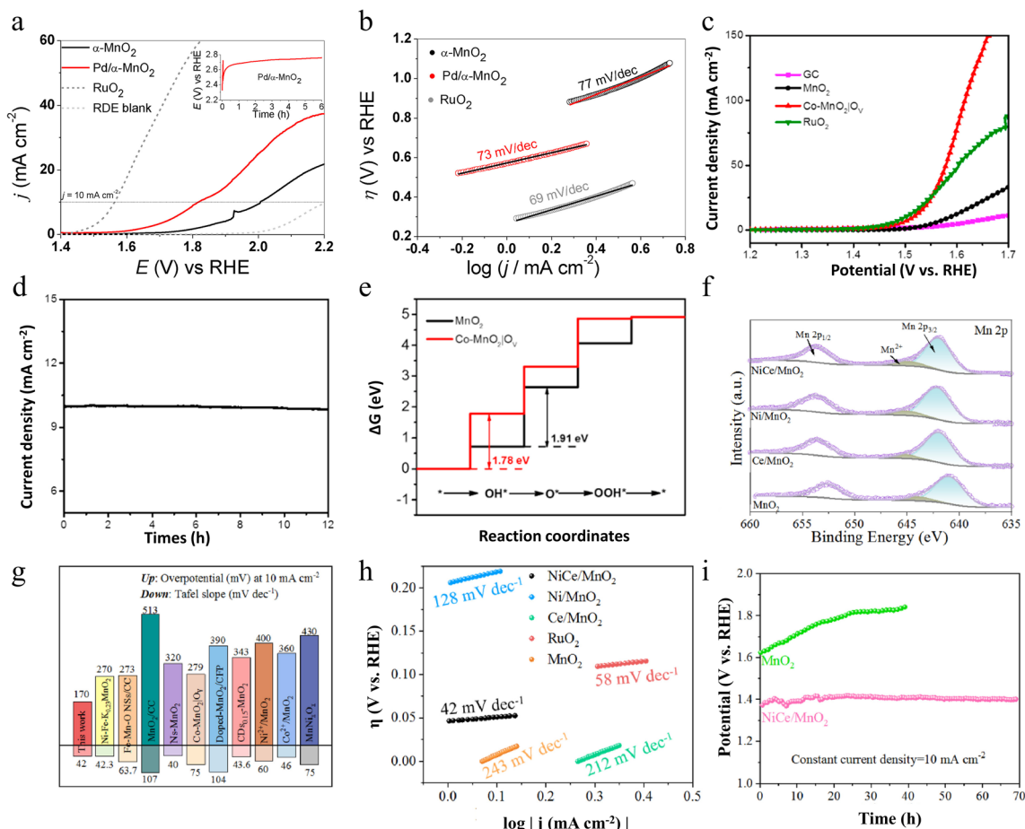
Fig. 10 The OER performance of Pd/ \alpha -MnO 2 , Co-MnO 2 |O v and NiCe/MnO 2 . (a) LSV curves and (b) Tafel plots of \alpha -MnO 2 , Pd/ \alpha -MnO 2 and RuO 2 . Reproduced with permission. 87 Copyright 2021, Elsevier. (c) Polarization curves and (d) time dependence of catalytic current density during electrolysis at a static potential of Co-MnO 2 |O v . (e) Reaction coordinates of the OER on MnO 2 and Co-MnO 2 |O v . Reproduced with permission. 88 Copyright 2018, Elsevier. (f) Mn 2p of MnO 2 , Ni/MnO 2 , Ce/MnO 2 and NiCe/MnO 2 . (g) Comparison with recently reported MnO 2 -based catalysts. (h) Tafel slopes and (i) the stability tests of NiCe/MnO 2 at 10 mA cm -2 of MnO 2 , Ce/MnO 2 , Ni/MnO 2 , NiCe/MnO 2 and RuO 2 . Reproduced with permission. 89 Copyright 2023, Elsevier.
