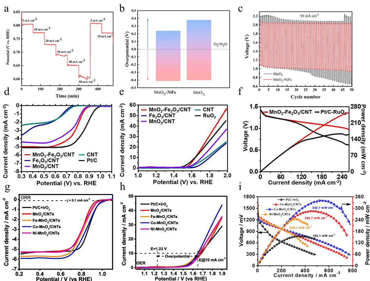
Fig. 17 The electrocatalytic performance of \text{MnO}_2 composites with metal/metal oxide materials. (a) Multitemporal potential curves of \text{MnO}_2 -NiFe prepared by a two-step electrodeposition method. (b) Chrono-potential plots at the current of 20 \text{ mA cm}^{-2} . (c) Stability test for \text{MnO}_2 -NiFe and \text{MnO}_2 at the current of 50 \text{ mA cm}^{-2} . Reproduced with permission. 130 Copyright 2019, American Chemical Society. (d) LSV curves for the ORR, (e) LSV curves for the OER, and (f) polarization curves and power density plots of \text{MnO}_2 - \text{Fe}_2\text{O}_3 /CNT prepared by spray pyrolysis and a subsequent bottom-up method and other samples. Reproduced with permission. 131 Copyright 2021, Elsevier. (g) ORR polarization curves, (h) OER polarization curves, and (i) the discharging polarization curves and power density plots for \text{M-MnO}_2 /CNTs (M: Fe, Co and Ni) prepared by a hydrothermal method and other samples. Reproduced with permission. 132 Copyright 2020, Elsevier.
