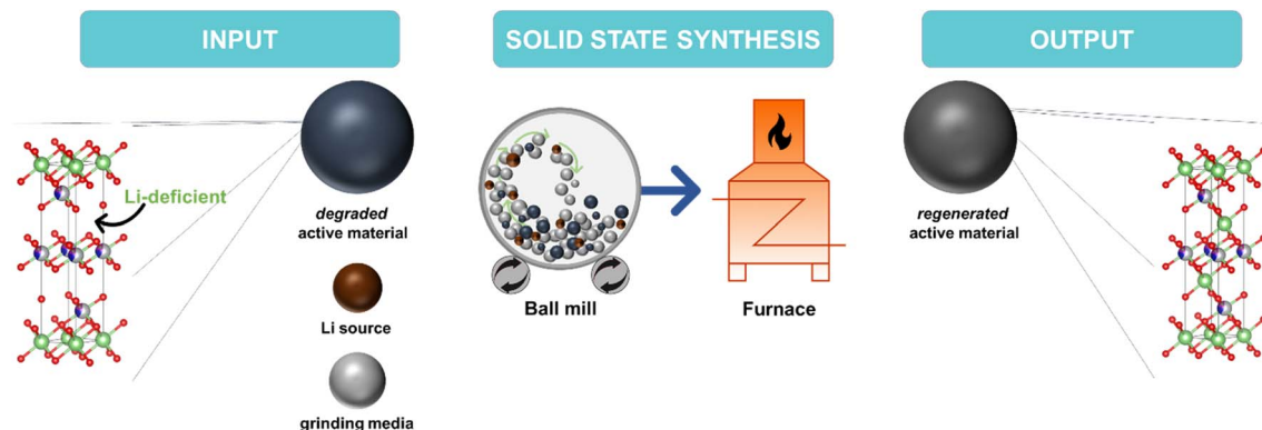
Fig. 10 Two-stage solid-state synthesis schematics: ball milling, followed by a heat treatment, to regenerate the layered oxide cathode active material.
