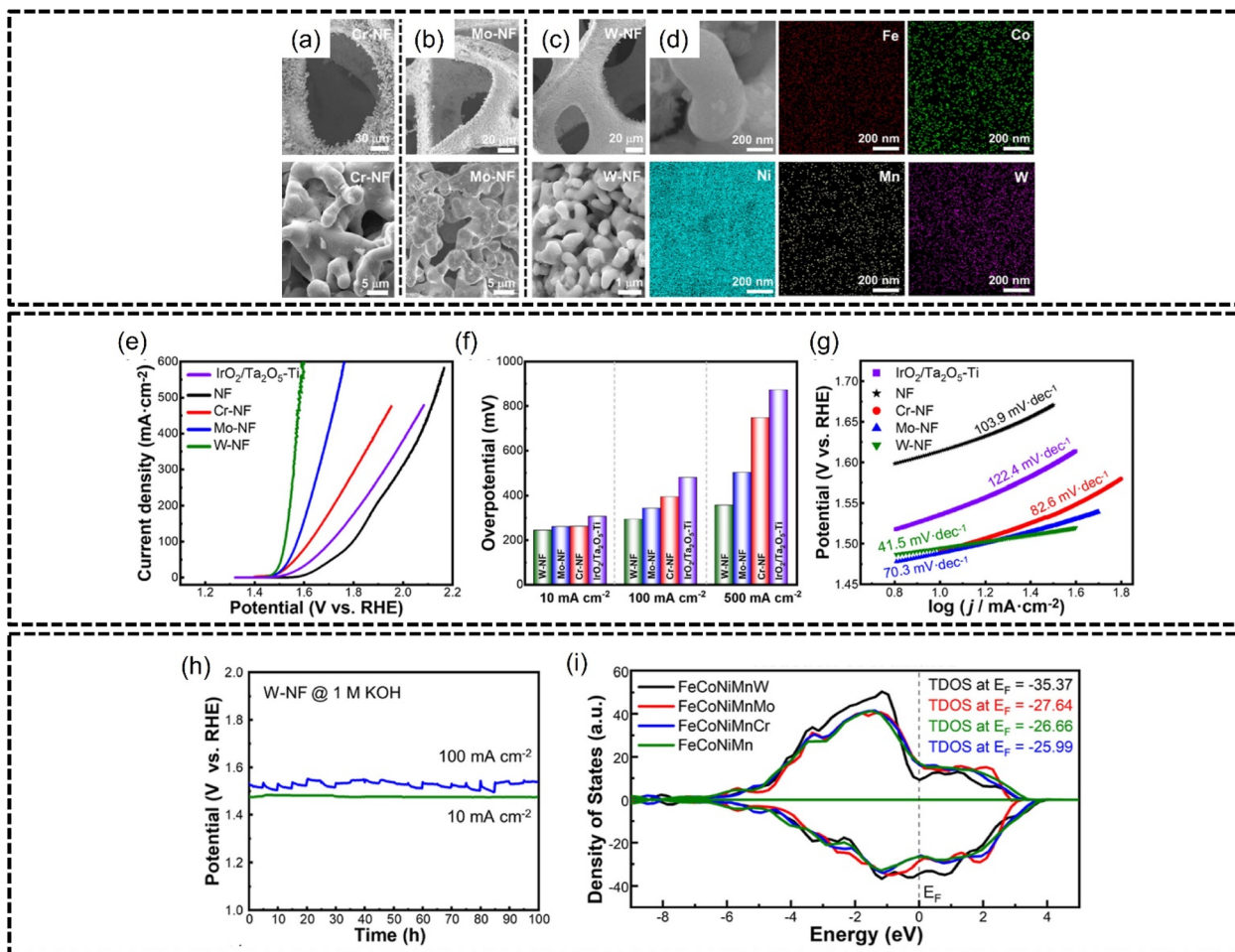
Fig. 15 FeCoNiMnW HEA characterization and OER performance based on the work of Li et al. Structural and morphological characterization. SEM images of (a) FeCoNiMnCr, (b) FeCoNiMnMo, and (c) FeCoNiMnW, on nickel foam, (d) EDX elemental mapping of FeCoNiMnW. Electrochemical measurements, (e) LSV curves, (f) OER overpotentials at 10, 100, and 500 mA cm -2 , (g) Tafel slopes, and (h) stability testing at 10 and 100 mA cm -2 for 100 h. (i) Total density of states plots for different electrodes. Reproduced with permission. 167 Copyright American Chemical Society 2023.
