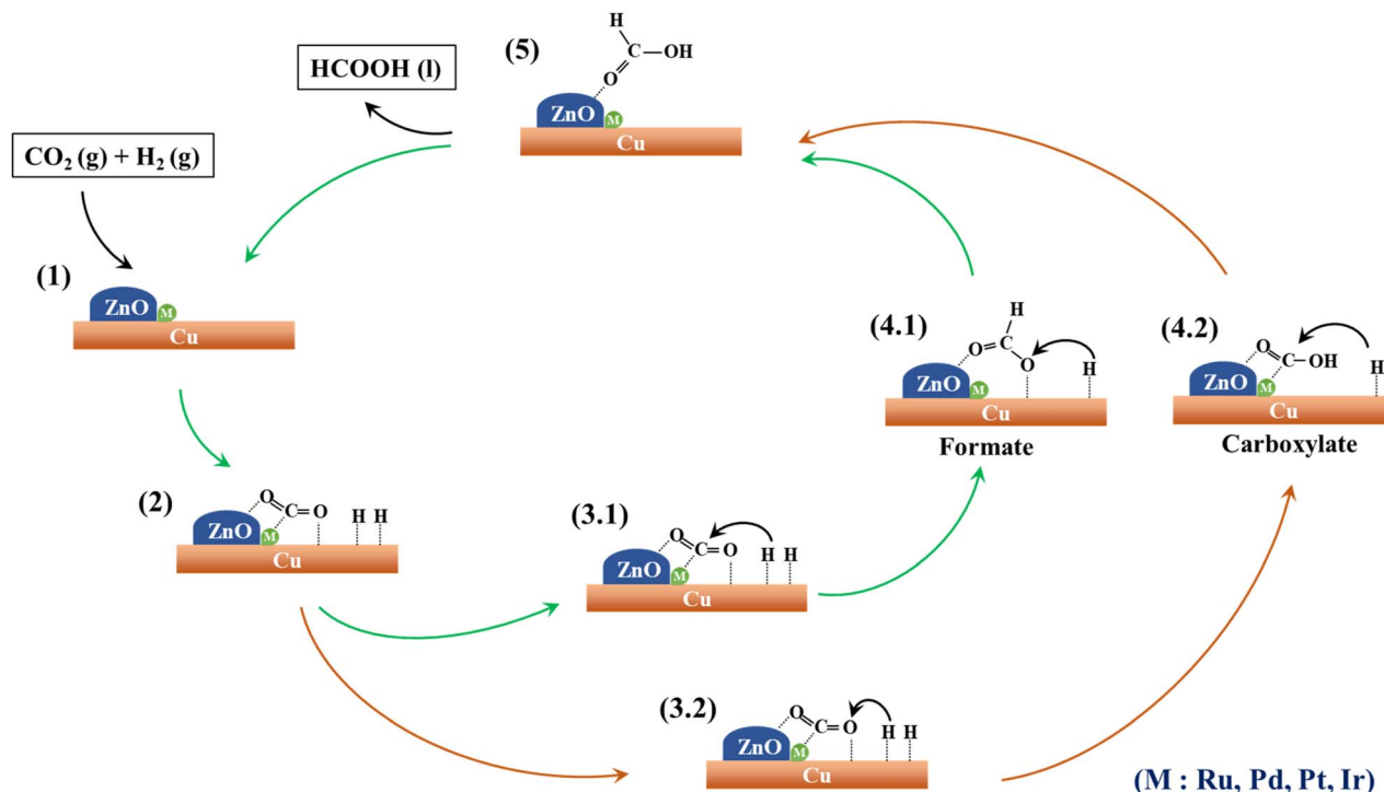
Fig. 9 A proposed mechanism for \text{CO}_2 hydrogenation to formic acid over the surface of M-CZ catalysts.
