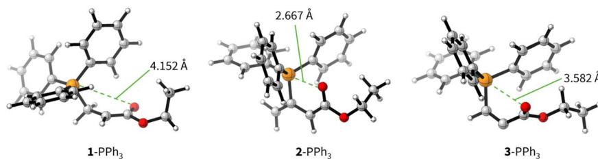
Fig. 11 Molecular structures of the zwitterionic adducts of PPh 3 with 1 , 2 , and 3 optimised at SMD(DCM)/MN15/def2-TZVPP level of theory. Green dashed lines indicate relevant P–O distances in the adducts.
