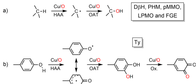
Scheme 1 Reaction type catalyzed by copper-containing mono-oxygenases (a) DβH (Dopamine β-monooxygenase); PHM (Peptidyl-glycine α-Hydroxylating Monoxygenase); pMMO (particulate Methane Monoxygenase); LPMO (Lytic Polysaccharide Monoxygenase); FGE (Formylglycine-Generating Enzyme) and (b) Ty (Tyrosinase).
