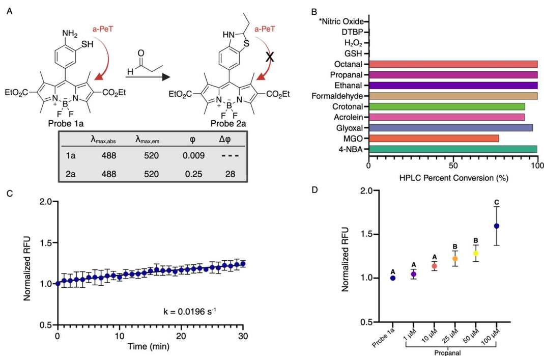
Fig. 2 (A) The reaction of 4-amino-3-thiophenol-BODIPY 1a with propanal generates dihydrobenzothiazole 2a activating the fluorescence by hindering the PeT process. The quantum yields calculation of probe 1a and dihydrobenzothiazole adduct 2a showed 28-fold increase in the fluorescence in DMSO and 80-fold increase in the aqueous conditions. (B) High chemoselectivity of probe 1a towards varying types of aldehydes generating dihydrobenzothiazoles. No product was formed with other biological metabolites. *Dithiol was produced with SNAP by-product. (C) Pseudo-first order rate constant of probe 1a with propanal is 0.0196 \text{s}^{-1} . (D) Limit of detection of probe 1a in detecting propanal in live T-47D cells. Letters indicate grouping by significance, P < 0.05 .
