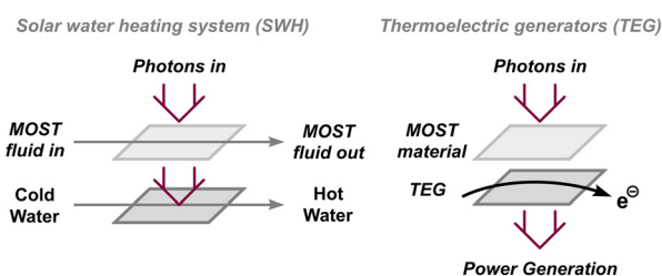
Fig. 7 Simplified schemes based on how SWH and TEG work when they are integrated with MOST systems.
