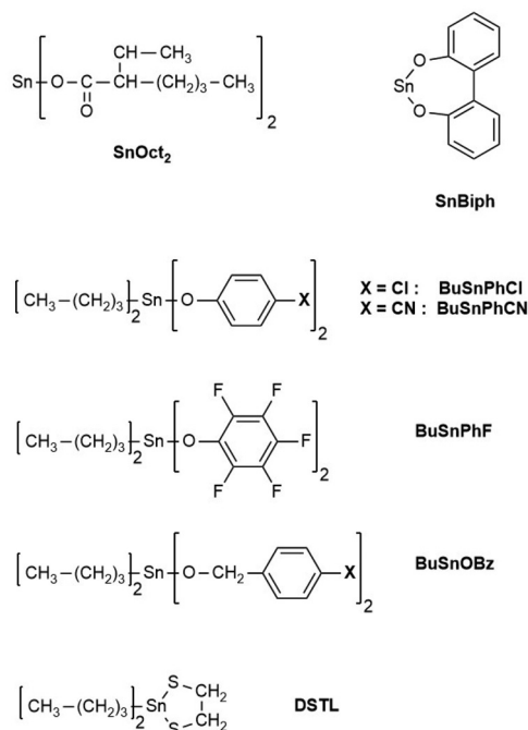
Scheme 3 Structure and acronyms of tin catalysts discussed in this work.
