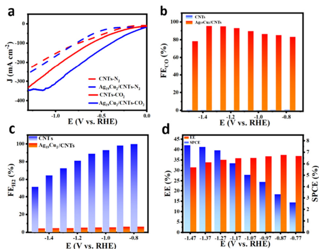
Fig. 3 (a) Polarization curve of CNTs and \text{Ag}_{19}\text{Cu}_2/\text{CNTs} in N 2 /CO 2 saturated 1 M KOH. (b) \text{FE}_{\text{CO}} of CNTs and \text{Ag}_{19}\text{Cu}_2/\text{CNTs} . (c) \text{FE}_{\text{H}_2} of CNTs and \text{Ag}_{19}\text{Cu}_2/\text{CNTs} . (d) EE and SPCE of the eCO 2 RR.
