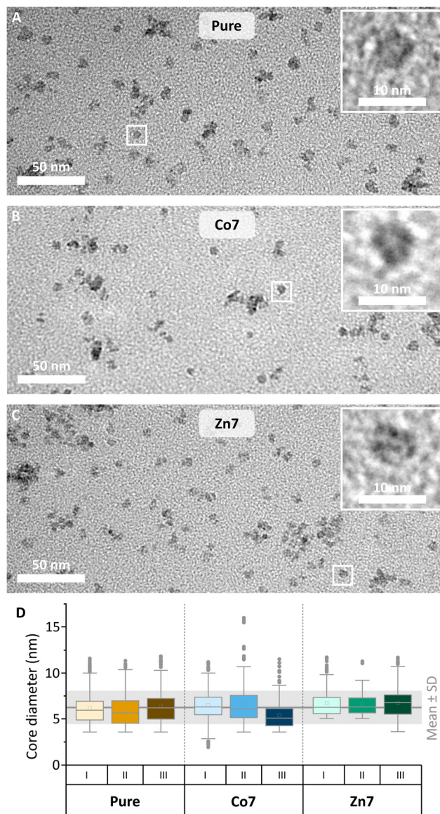
Fig. 2 (A–C) Transmission electron microscopy images of magnetoferri-feritin. Images of all doping conditions were taken without staining to visualise metallic cores. (D) Box plots showing the diameters of cores from three independent synthesis runs (I, II and III) of all three doping conditions (each N \geq 93 ; mean \pm SD = 6.3 \pm 1.8 nm). Mean values are shown as boxes and median values are shown as horizontal lines.
