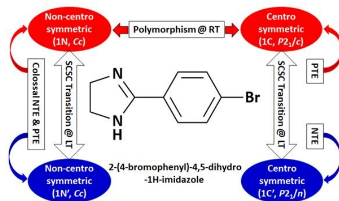
Figure 16: Polymorphism, phase transition, and unusual thermal expansion characteristics in halogen derivatives of 4-phenyl substituted imidazoline. 168
