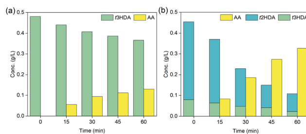
Fig. 5 Concentration ( \text{g L}^{-1} ) of trans -2-hexenedioic acid (t2HDA), trans -3-hexenedioic acid (t3HDA) and adipic acid (AA) with reaction time (min) for constant-current ( -100 mA) bulk electrolysis using (a) t3HDA, and (b) HDA mix model solutions on Pd/C.
