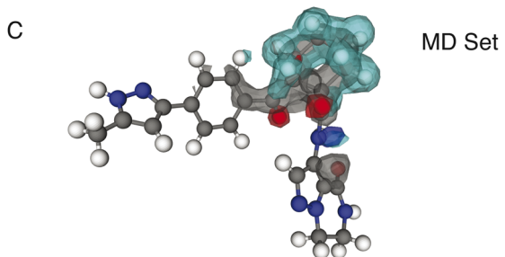
Fig. 3 (A) Histogram of dihedral angles for the C14–C19 bond in the MD set (blue) and NMR set with all shifts (red). (B and C) Three-dimensional atomic density maps aligned about the C14–C19 bond showing the density for the NMR set (B) and the MD set (C). The colors gray, blue, teal, and red represent carbon, nitrogen, hydrogen, and oxygen, respectively.
