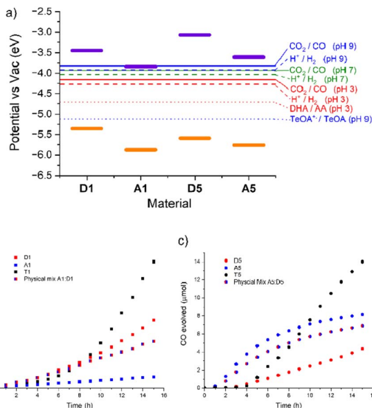
Fig. 2 (a) IPs (orange) and EAs (purple) of the materials along with relevant electrochemical potentials. (b) Photocatalysis of the Co-loaded group 1 polymers (2.5 mg) and 2,2'-bipyridine (2 mg) in MeCN : water (6 : 1, 35 mL) with Ascorbic acid (616 mg) under an atmosphere of CO 2 . (c) Photocatalysis of the Co-loaded group 5 polymers (2.5 mg) and 2,2'-bipyridine (2 mg) in MeCN (32 mL) with TeOA (3 mL) under an atmosphere of CO 2 .
