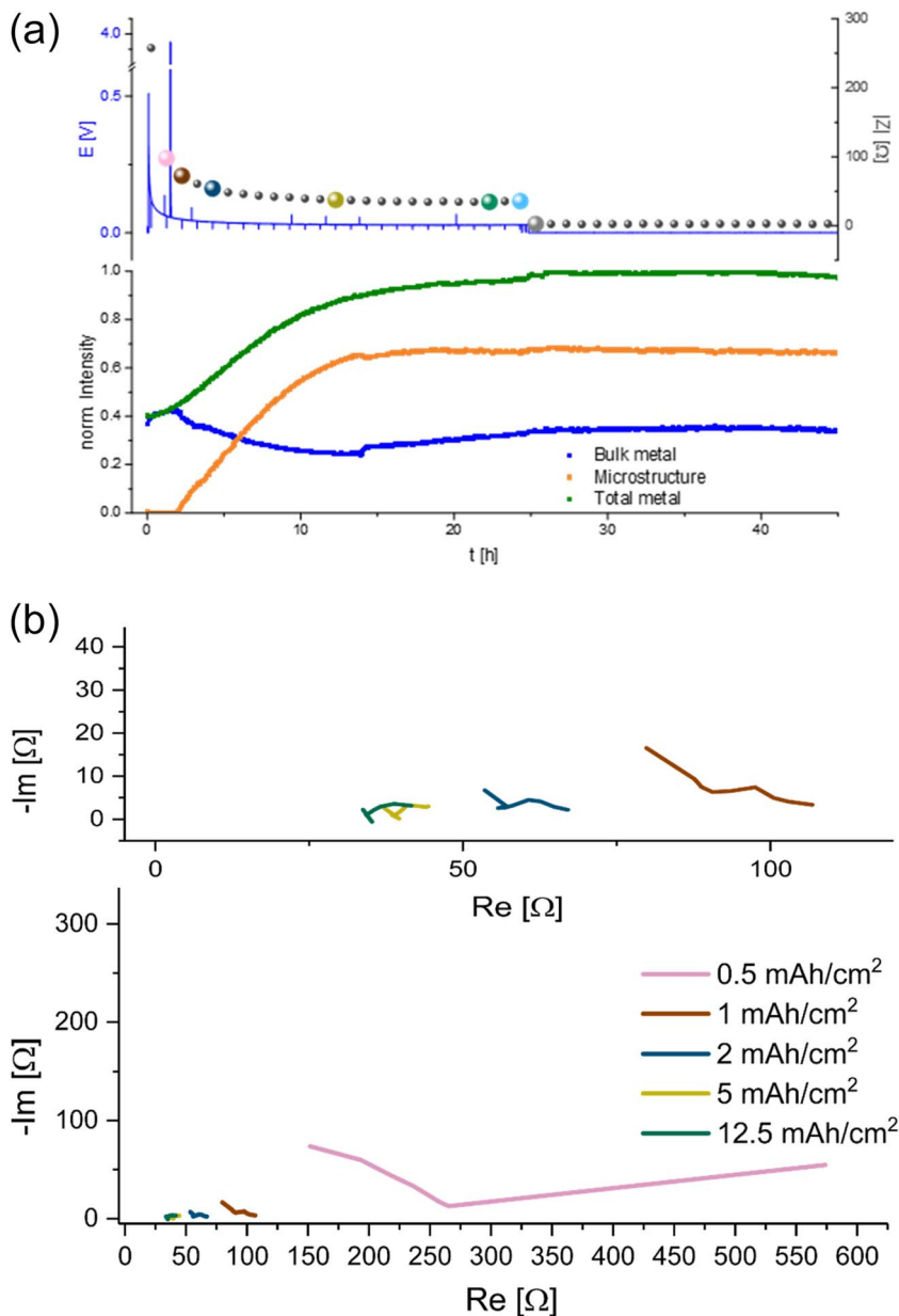
Fig. 9 (a) Operando ^7Li NMR and impedance (GEIS) measured at 9 Hz. Intensities measured during unidirectional Li plating at 1 mA cm^{-2} in an NMR in situ cylindrical symmetrical Li cell with LP30 + 10% FEC electrolyte. (b) GEIS Nyquist plots measured with 100 \mu A amplitude during Li plating at 1 mA cm^{-2} in an NMR in situ cylindrical symmetric cell, using LP30 + FEC electrolyte with GF separator at RT. Magnification of the plot at 5–15 mA h cm^{-2} .
