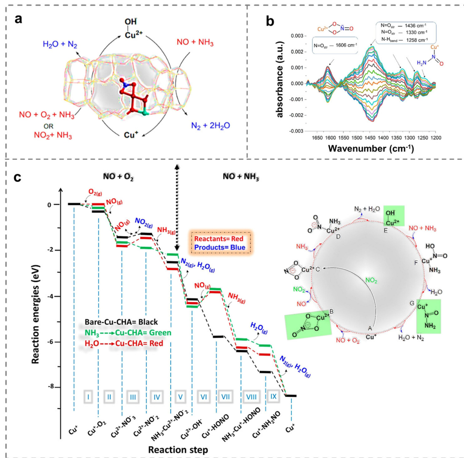
Fig. 3 (a) Schematic of the \text{NH}_3 -SCR reaction mechanism on Cu-SSZ-13 zeolites. (b) Concentration modulation ME DRIFTS experiment with the corresponding phase-resolved spectrum. (c) Reaction mechanisms on the bare active site (black), ammonia-physorbed active site (green) and water-physorbed active site (red). Copied with permission from ref. 76. Copyright 2022, American Chemical Society.
