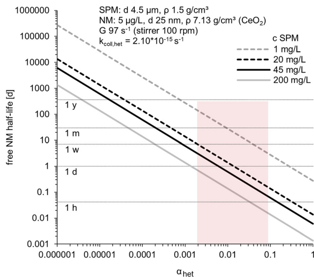
Fig. 5 Pseudo-first-order free NM half-life in dependence of \alpha_{\text{het}} calculated for different SPM concentrations ( c_{\text{SPM}} : 1, 20, 45, 200 mg \text{L}^{-1} ) setting the parameters to represent the experiments ( i.e. , for SPM: diameter 4.5 \mu\text{m} , density 1.5 \text{g cm}^{-3} ; for NM: concentration 5 \mu\text{g L}^{-1} , diameter 25 nm, density of \text{CeO}_2 7.13 \text{g cm}^{-3} ; assuming spherical shape for both; velocity gradient G 97 \text{s}^{-1} for 100 rpm stirring). Black lines indicate the SPM concentrations used in the experiments, and the shaded area highlights the range of \alpha_{\text{het\_size-dis}} values determined (see Fig. 3).
