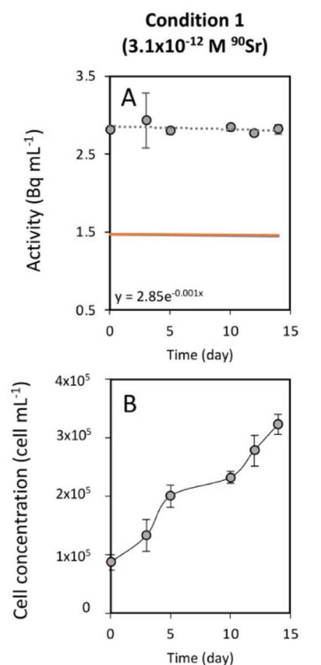
Fig. 2 (A) Time evolution of the activity measured in the growth medium of T. marina cultures amended with 3.1 \times 10^{-12} \text{ M } ^{90}\text{Sr} . Grey circles correspond to the total activity of the culture medium. The dashed line represents the calculated exponential reduction fit of the total activity. Its associated equation is expressed on the bottom left area of the graph. The orange line corresponds to the estimated ^{90}\text{Y} activity and the blue line to the estimated ^{90}\text{Sr} activity. In this case, both lines are superposed. (B) Time evolution of the cell concentration of T. marina cultures amended with 3.1 \times 10^{-12} \text{ M } ^{90}\text{Sr} . The error bars represent the standard deviations ( n = 3 ).
