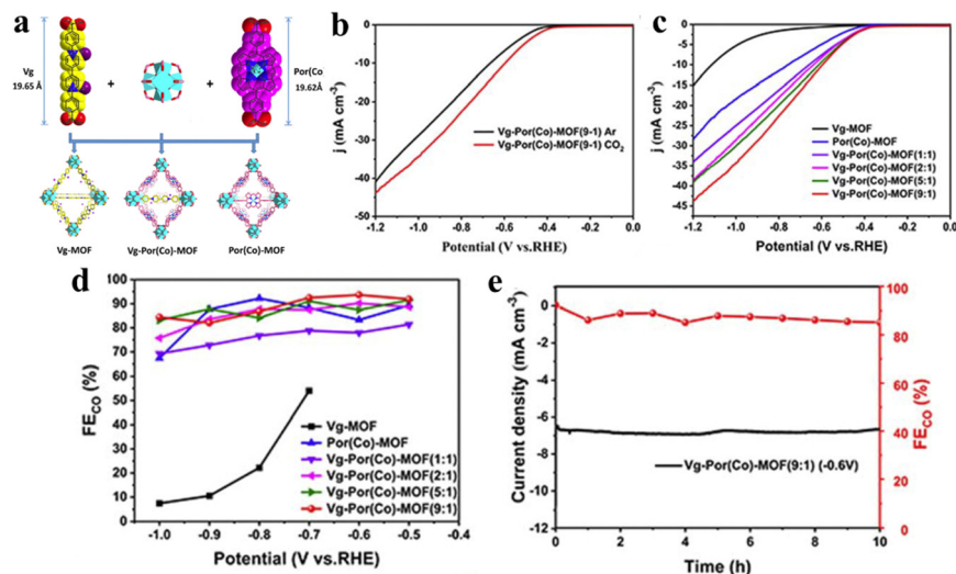
Fig. 16 (a) Schematic of the synthesis of Vg-MOF, Por(Co)-MOF, and Vg-Por(Co)-MOF by the solvothermal method. (b) LSV curves of Vg-Por(Co)-MOF (9 : 1) in \text{CO}_2 - and Ar-saturated 0.5 M \text{KHCO}_3 . (c) LSV curves of Vg-MOF, Por(Co)-MOF and Vg-Por(Co)-MOF ( n : 1) ( n = 1, 2, 5, 9) in a 0.5 M \text{KHCO}_3 electrolyte under \text{CO}_2 . (d) Faradaic efficiencies of CO for Vg-MOF, Por(Co)-MOF and Vg-Por(Co)-MOF ( n : 1) ( n = 1, 3, 5, 9). (e) Stability of Vg-Por(Co)-MOF (9 : 1) at a potential of -0.6 V versus RHE for 10 h. Reproduced from ref. 147. Copyright 2022 RSC.
