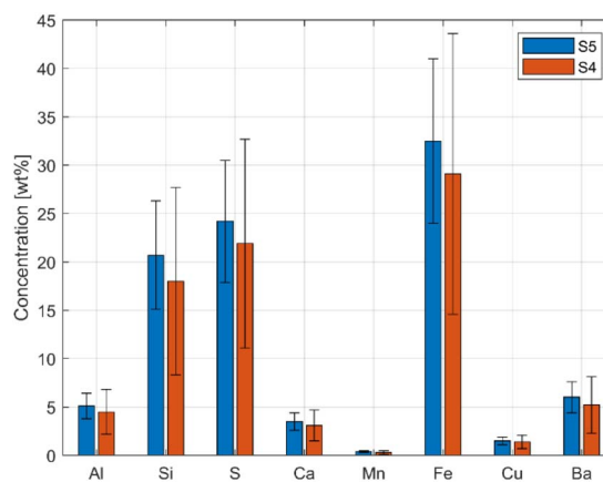
Fig. 10 Concentration expressed as weight percentage (wt%) of inorganic fractions detected in the collected particulates.
