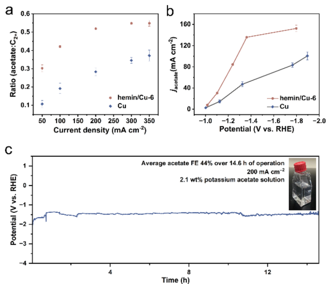
Fig. 3 Acetate production performance of hemin/Cu-6 and Cu NPs. (a) The ratio of acetate to \text{C}_{2+} products (ethylene, ethanol, acetate, and n -propanol) for the hemin/Cu-6 and Cu catalysts at different applied currents. (b) Partial current density of acetate for the hemin/Cu-6 and Cu catalysts at different applied potentials. (c) Chronopotentiometry stability test of hemin/Cu-6 using a flow cell at 200 \text{ mA cm}^{-2} in 1 M \text{KHCO}_3 with a product concentration of 2.1 wt% (0.235 M).
