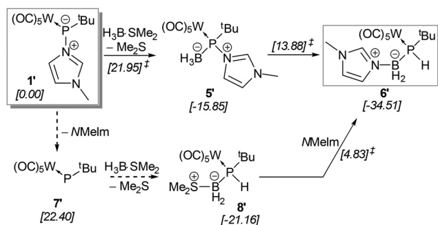
Scheme 4 Proposed mechanism for the formation of the rearranged model product 6' from phosphinidene adduct complex 1' . The computed [CPCM THF /PWBP95-D3/def2-QZVPP/CPCM THF /PBEh-3c] relative Gibbs free energies ( \text{kcal mol}^{-1} ) are given in square brackets for ground and transition states (the latter indicated by the ‡ superscript). The dashed arrows indicate barrierless processes.
