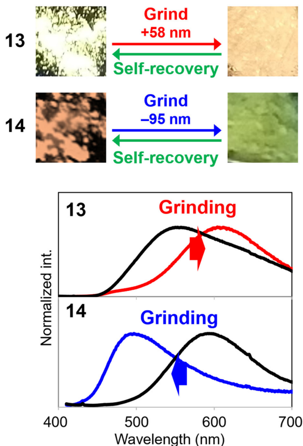
Fig. 6 Mechanochemical luminescence and self-recovery of 13 and 14 . Reprinted with permission from ref. 34. Copyright 2023 Wiley-VCH Verlag GmbH & Co. KGaA, Weinheim.
