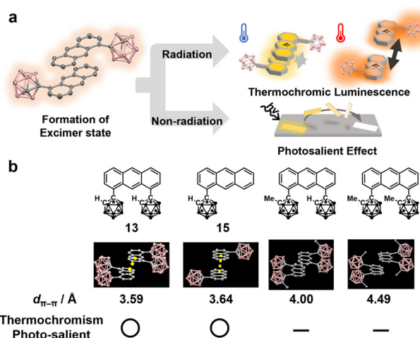
Fig. 8 (a) Schematic illustration of photochemical processes from the excimer state. (b) Structure and property relationship on the photosalient effect based on the o -carborane-modified anthracene derivatives. Reprinted with permission from ref. 41. Copyright 2024 Wiley-VCH Verlag GmbH & Co. KGaA, Weinheim.
