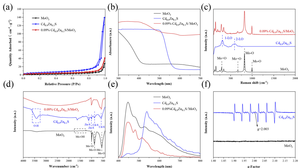
Fig. 3 (a) \text{N}_2 adsorption–desorption isotherms, (b) UV-vis DRS, (c) Raman spectra, (d) FTIR spectra, (e) PL spectra, and (f) EPR spectra of \text{MoO}_3 , \text{Cd}_{0.9}\text{Zn}_{0.1}\text{S} and 0.09\% \text{ Cd}_{0.9}\text{Zn}_{0.1}\text{S}/\text{MoO}_3 .
