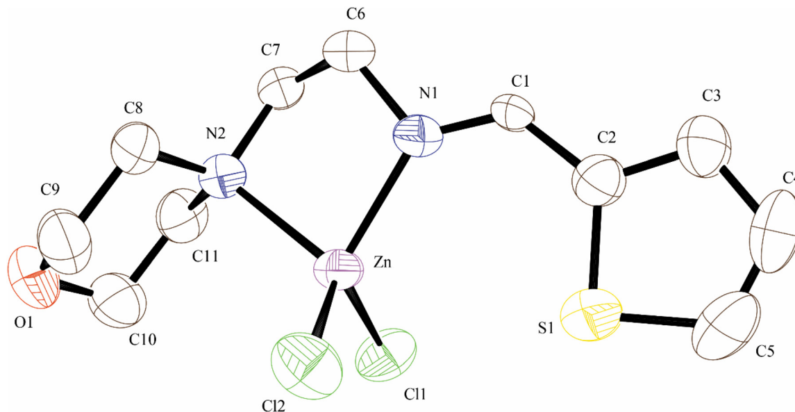
Fig. 3 Molecular structure of [\text{TEM}(\text{Zn})\text{Cl}_2] with thermal ellipsoids at 60% probability.
