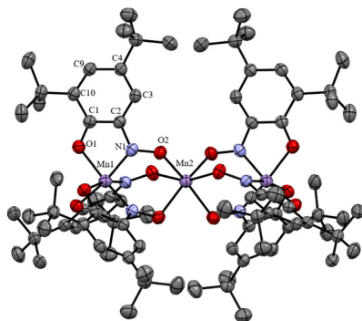
Fig. 1 Molecular structure of \{[MnL_3]Mn[MnL_3]\} ( 1 ) according to the SCXRD data (hydrogen atoms are not shown). Only symmetry non-equivalent atoms are labelled.
