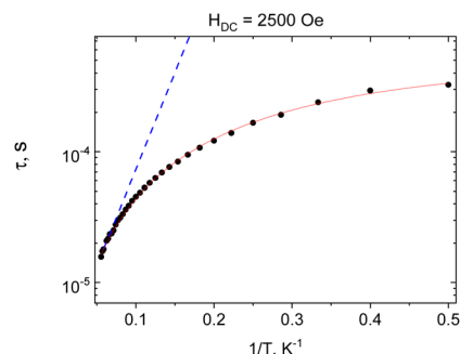
Fig. 5 Dependence of the relaxation time and the inverse of temperature ( 1/T ) of 1 ( H_{\text{DC}} = 2500 \text{ Oe} ). Blue dotted line – approximation of the high temperature part by the Arrhenius law. Red solid line – approximation by the sum of Raman and QTM-type contributions. Black circles – experimental data.
