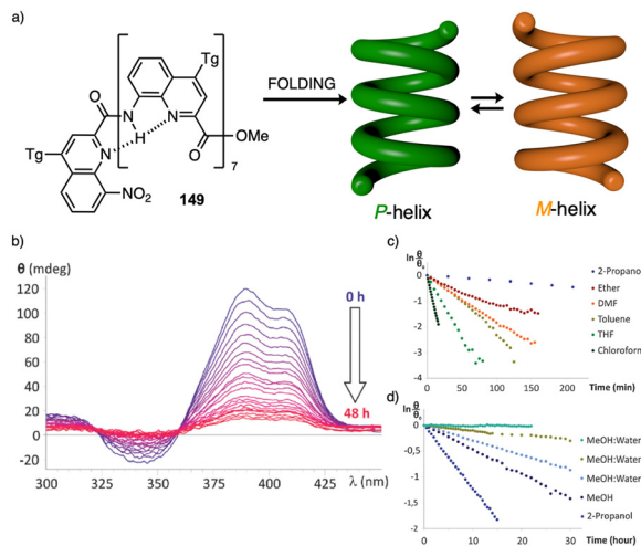
Fig. 71 (a) Chemical structure of foldamer 149 and its folding into a mixture of P - and M -helices. Time dependent ECD racemization studies for P - 149 as a function of solvent in (b) MeOH, (c) different solvents and (d) MeOH:Water mixtures. Reproduced from ref. 354 with permission from the Royal Society of Chemistry, copyright 2012.
