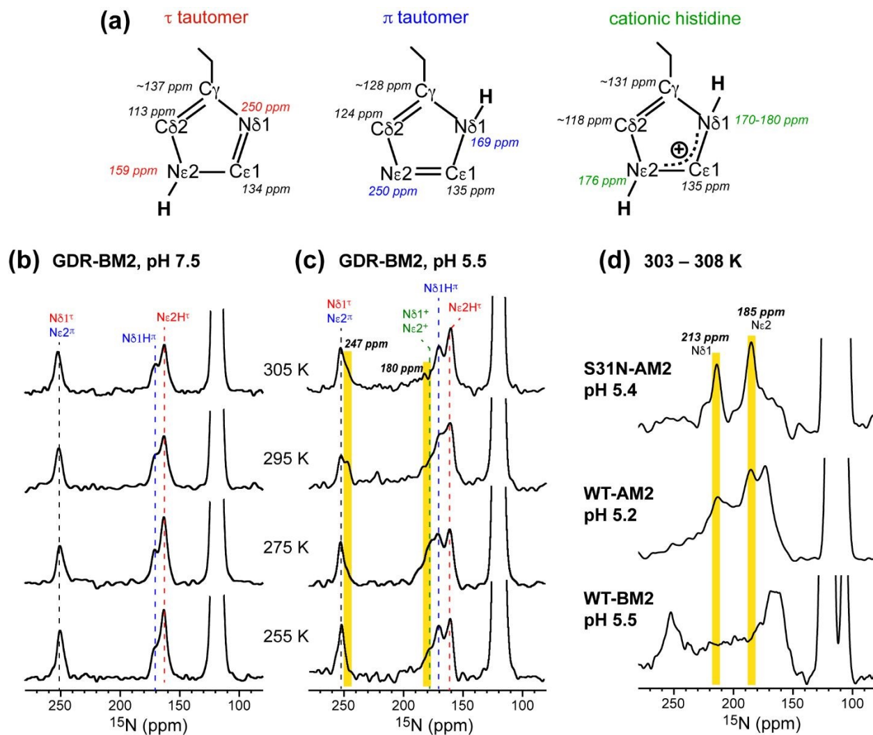
Figure 2. Variable-temperature ^{15}\text{N} CP spectra of membrane-bound GDR-BM2 at neutral and acidic pH from 255 K to 305 K. (a) Canonical ^{13}\text{C} and ^{15}\text{N} chemical shifts of the three histidine structures based on previous studies of M2 proteins 21, 52 and amino acid histidine 37 . (b) ^{15}\text{N} spectra of GDR-BM2 at pH 7.5. (c) ^{15}\text{N} spectra of GDR-BM2 at pH 5.5. (d) Previously reported high-temperature ^{15}\text{N} spectra of S31N-AM2 47 , WT-AM2 22 , and WT-BM2 24 around pH 5.5. The \tau tautomer, \pi tautomer, and cationic histidine signals are assigned in red, blue, and green, respectively. Yellow shaded bars denote exchange peaks observed at high temperature in the pH 5.5 samples. In all figures, the indicated temperatures of GDR-BM2 are set temperatures for the NMR probe. The estimated sample temperatures are listed in Table S1.
