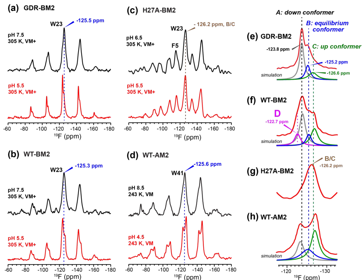
Figure 7. ^{19}\text{F} CP spectra of 5- ^{19}\text{F} -Trp in M2 peptides resolve multiple Trp conformations at acidic pH. For each peptide, two samples were measured, at neutral pH (6.5–8.5) and acidic pH (4.5–5.5). Panels (e–h) are zoomed-in centerband regions of the acidic-pH spectra in panels (a–d), to better display the partially resolved peaks. Dashed lines guide the eye for the different ^{19}\text{F} chemical shifts. (a) ^{19}\text{F} spectra of W23 in GDR-BM2 measured at 305 K. The neutral-pH spectrum shows a single broad peak whereas the acidic-pH spectrum resolves three peaks (A: -123.8 ppm; B: -125.2 ppm; C: -126.6 ppm), as shown in (e). (b) ^{19}\text{F} spectra of W23 in WT-BM2. The neutral-pH spectrum shows a single broad peak while the acidic-pH spectrum resolves four components (A: -124.1 ppm; B: -125.5 ppm; C: -126.8 ppm; D: -122.7 ppm), as shown in (f). (c) ^{19}\text{F} spectra of W23 in H27A-BM2. Both the neutral pH and acidic pH spectra show a single broad peak. The latter spectrum's centerband is shown in (g). This peptide also contains 4- ^{19}\text{F} -labeled Phe5 with an isotropic shift of -116 ppm. (d) Low-temperature ^{19}\text{F} CP spectra of membrane-bound WT-AM2 at pH 8.5 and pH 5.5, adapted from 16 . The pH 4.5 spectrum resolves three peaks (A: -123.5 ppm; B: -125.4 ppm; C: -127.2 ppm), as shown in (h). Peaks A, B, and C are assigned to a down conformer, an equilibrium conformer, and an up conformer of the indole ring based on an integrated analysis of these spectra and on the structure and dynamics of W41 in AM2 16 .
