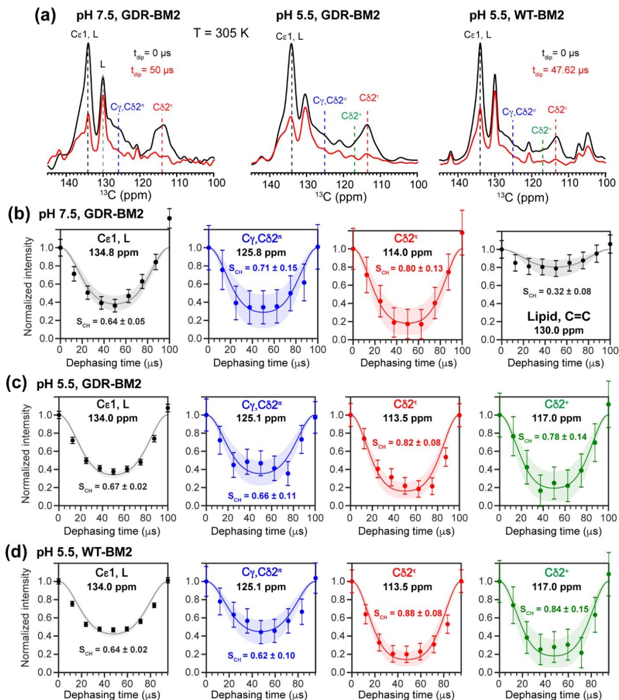
Figure 6. 2D ^{13}\text{C} - ^1\text{H} DIPSHIFT data of membrane-bound GDR-BM2 and WT-BM2. The spectra were measured at 305 K under 10 kHz or 10.5 kHz MAS. (a) Aromatic region of the ^{13}\text{C} dimension of the 2D spectra of the three peptides at C-H dipolar evolution times of 0 \mu\text{s} and half of the rotor period (50 \mu\text{s} or 47.6 \mu\text{s} ). (b) C-H dipolar dephasing of GDR-BM2 at pH 7.5. (c) C-H dipolar dephasing of GDR-BM2 at pH 5.5. (d) C-H dipolar dephasing of WT-BM2 at pH 5.5. Error bars were propagated from the spectral signal-to-noise ratios. Best-fit simulations (solid lines) are shown along with uncertainties in the S_{\text{CH}} values (shaded areas) up to two standard deviations. The rigid-limit C-H dipolar coupling is assumed to be 23.9 kHz.
