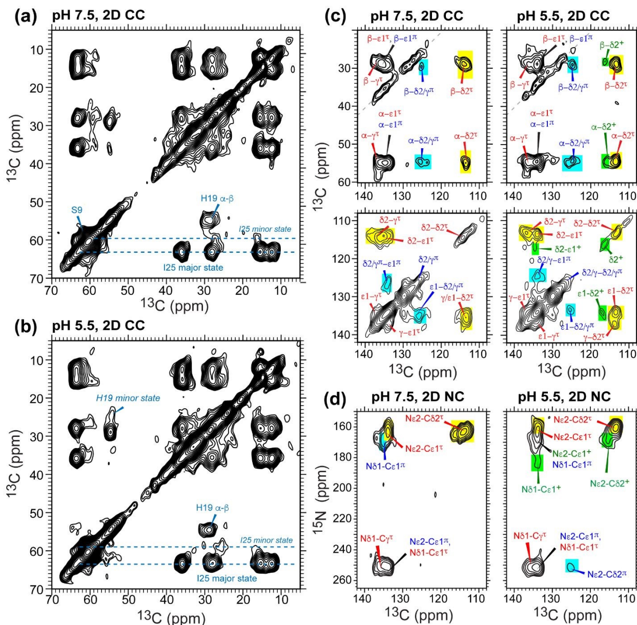
Figure 4. 2D ^{13}\text{C} - ^{13}\text{C} and ^{15}\text{N} - ^{13}\text{C} correlation spectra of membrane-bound GDR-BM2 to resolve tautomeric and cationic H19 species. (a) 2D CC spectrum at pH 7.5. (b) 2D CC spectrum at pH 5.5. Resonance assignment of the \tau tautomer, \pi tautomer, and cationic His is shown in red, blue and green, respectively. (c) Aromatic region of the 2D CC spectra. (d) Aromatic region of the 2D NC spectra. Colored boxes indicate the integration areas for intensity quantification to obtain the percent populations of \tau (yellow), \pi (cyan) and cationic (green) histidine. The spectra were measured at 255 K.
