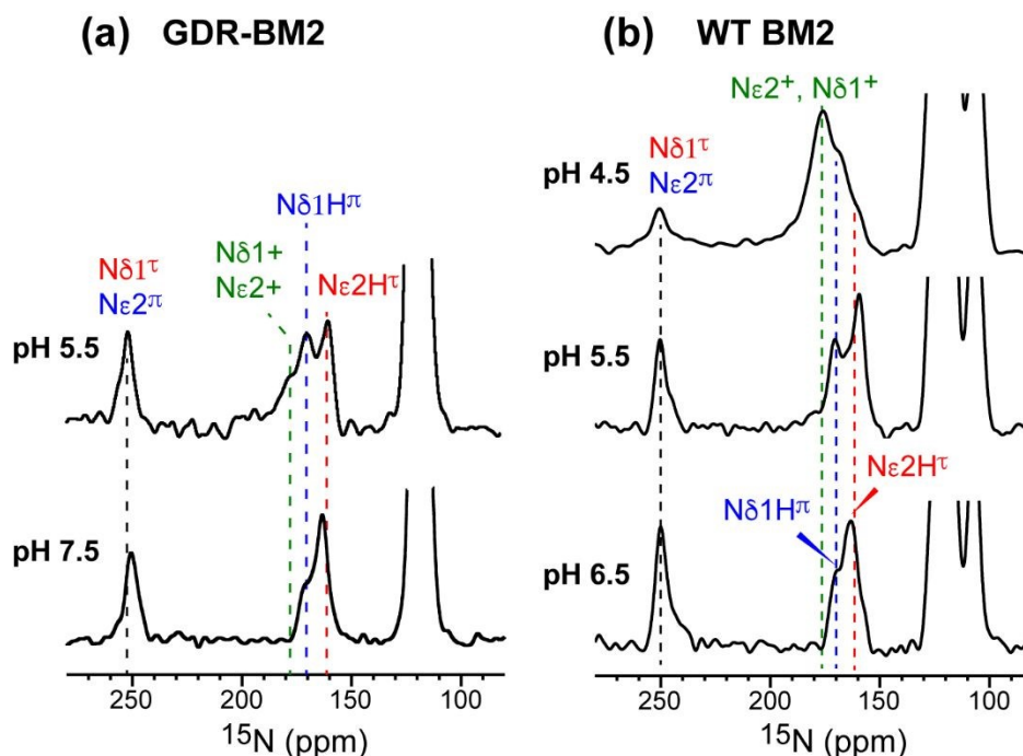
Figure 3. ^{15}\text{N} spectra of membrane-bound GDR-BM2 and WT-BM2 measured at 255 K. (a) Spectra of GDR-BM2 at pH 7.5 and pH 5.5. (b) Previously reported spectra of WT-BM2 at pH 6.5, 5.5 and 4.5 16 . Between pH 6.5 and 7.5, the two peptides exhibit similar ^{15}\text{N} chemical shifts and intensity distributions, indicating similar populations of \tau and \pi tautomers. At pH 5.5, GDR-BM2 exhibits higher cationic His intensities than WT-BM2, indicating that the GDR mutant channel stabilizes the cationic histidine. At pH 4.5, WT-BM2 shows predominantly cationic His intensities.
