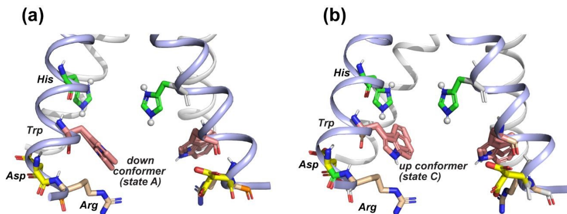
Figure 8. Provisional model of the tryptophan sidechain conformation that regulates the interactions of this residue with the N-terminal proton-selective histidine and the C-terminal charged residues. The crystal structure of AM2 at pH 5.5 (PDB: 4QKM) is used for modeling 29 . Key residues (H37, W41, D44 and R45) in two neighboring chains (light blue) are shown as sticks. H37 is cationic in this crystal structure. (a) A putative tryptophan down conformer (state A) that interacts with the C-terminal charged residues. The Trp ( \chi_1 , \chi_2 ) torsion angles in the left chain are slightly modified to (-175^\circ, -75^\circ) from the original structure. The original structure has Trp ( \chi_1 , \chi_2 ) torsion angles of (-175^\circ, -90^\circ) , which are shown in the chain on the right. (b) A putative tryptophan up conformer (state C) that interacts with the cationic histidine. The Trp ( \chi_1 , \chi_2 ) torsion angles in the left chain are modified to (-155^\circ, +135^\circ) from the original structure to depict this state.
