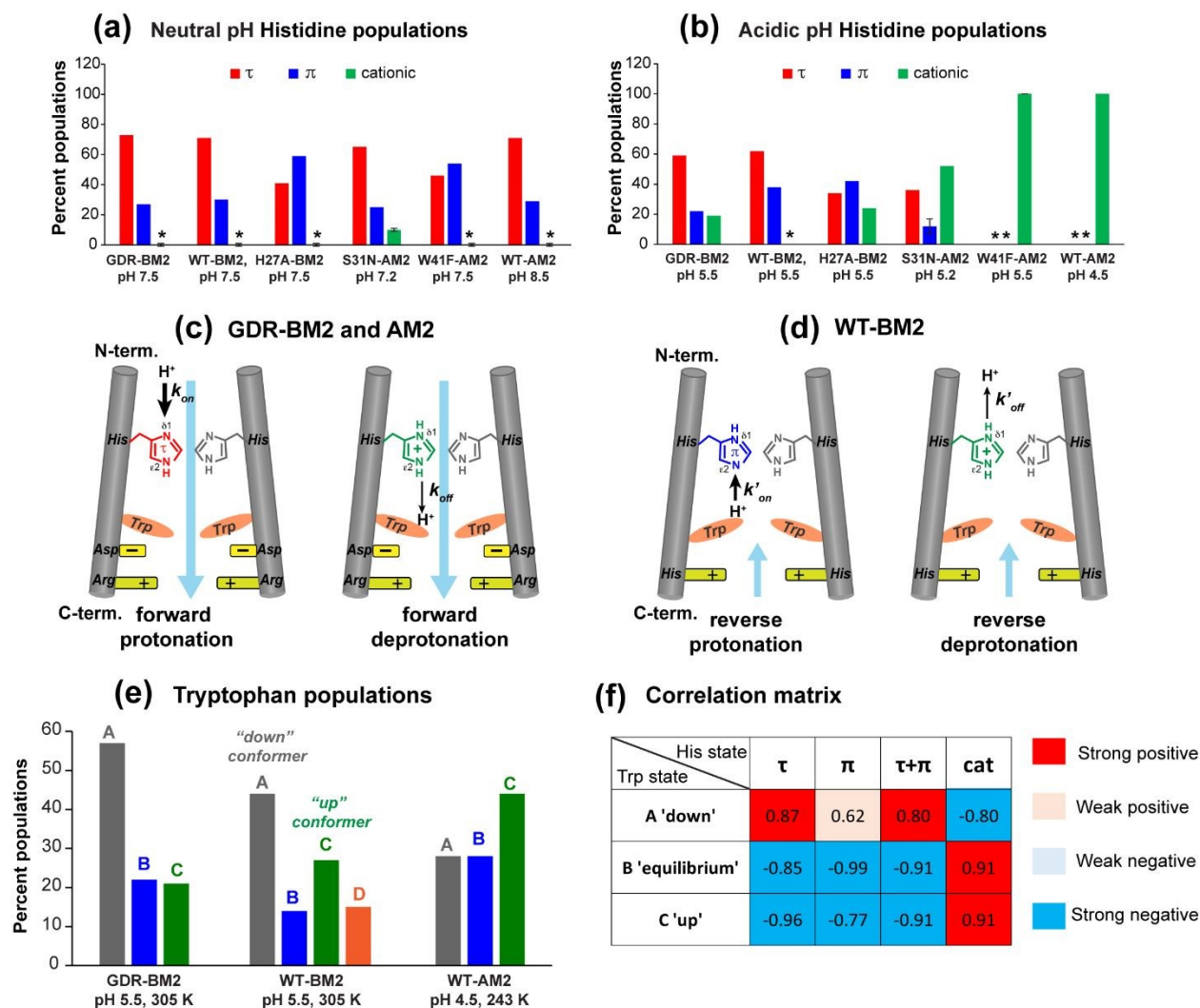
Figure 5. Percent distributions of histidine and tryptophan states for various M2 peptides. (a) Distributions of histidine structures at pH 7.5. (b) Distribution of histidine structures at pH 5.5. These populations are obtained from spectral intensities listed in Table S3. Asterisks indicate 0% populations. (c) Schematic of the main proton transfer processes in inward-rectifying AM2 and GDR-BM2 channels. Only two out of four helices are represented for clarity. The charge state of the histidine on the left is specifically indicated whereas the charge state of the histidine on the right is independent and is shown in grey. The charged residues C-terminal to Trp are Asp and Arg in these channels. Forward deprotonation at acidic pH is facilitated by increased water accessibility around the gating complex. Blue arrow denotes inward proton conduction in these channels. (d) Schematic of the additional proton transfer pathways in WT-BM2. The charged residue C-terminal to Trp is a His. Reverse protonation is facilitated by increased water accessibility around the gating complex. Blue arrow denotes the fact that WT-BM2 conducts protons from the C-terminus to the N-terminus when \text{pH}_{\text{in}} is acidic. This outward conduction is additional to the inward conduction that is similar to (c). (e) Distributions of Trp conformations obtained from the ^{19}\text{F} NMR spectra. (f) Pearson correlation matrix between His and Trp states for GDR-BM2, WT-BM2 and WT-AM2 at acidic pH.
