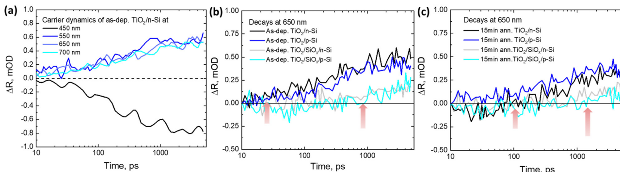
Fig. 5 (a) Extracted charge transfer dynamics after excitation of the HF-treated as-dep. \text{TiO}_2/\text{n-Si} sample at 500 nm (with 200 \mu\text{J cm}^{-2} energy density) where the increase of the signal at different wavelengths is shown as a function of time which corresponds to the charge transfer signal increase at different wavelengths, and comparison of the extracted charge transfer signal increase at 650 nm probe wavelength for all the (b) HF-treated as-dep. \text{TiO}_2/\text{Si} samples, and (c) 15 minute annealed \text{TiO}_2/\text{Si} samples. The red arrow shows the charge transfer onset time where the charge transfer signal from Si to \text{TiO}_2 first appears above the noise range.
