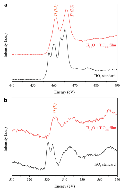
Fig. 8 Electron energy loss spectra of (a) Ti L_{2,3} and (b) O K edge of the r\text{-}Ti_{1-x}O + r\text{-}TiO_{2-x} predominant thin film as deposited on the FTO-coated silica glass by the PLA process under 600 mJ per pulse in vacuum (red traces) in comparison with the rutile TiO_2 standard (black traces, EELS Atlas, Gatan Inc.).
