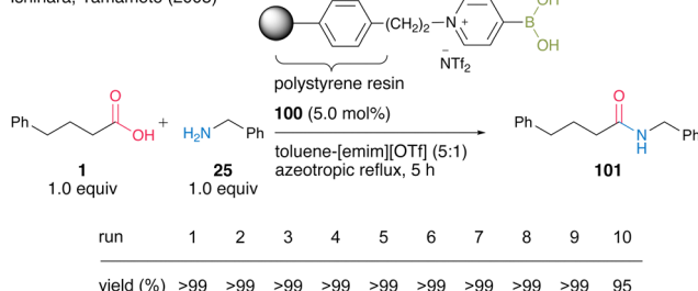
Scheme 18 Polymer-supported 4-pyridinium boronic acid-catalyzed amidation reported by Ishihara and Yamamoto. 34
