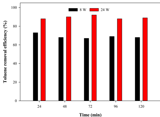
Fig. 4 Photocatalytic activity of the paint P-3 under 8 W and 24 W white light against 3 ppm toluene at a total flow rate of 50 mL min -1 .
