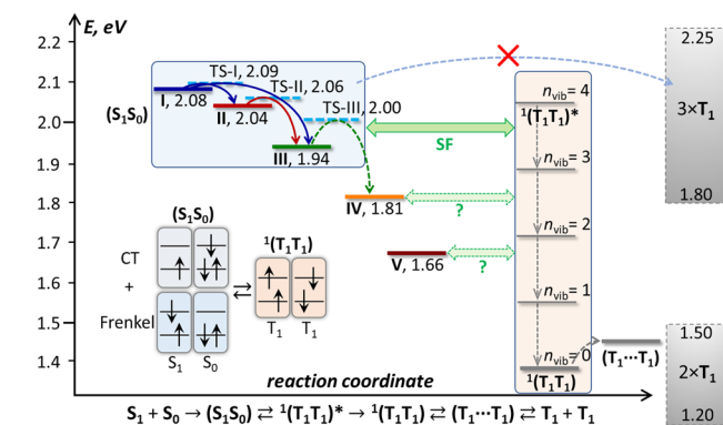
Fig. 9 Schematic energy diagram of the excited states in DBP single crystal. Emissive states I–V found in PL measurements are shown in colors corresponding to the spectra in Fig. 5, and the transition state levels (TS-I, TS-II, TS-III) are shown as dashed cyan lines. The triplet state energy of DBP is not well known; a conservative estimation places it between 0.60 and 0.75 eV, hence 2 \times T_1 and 3 \times T_1 levels are depicted as rectangles spanning possible energy ranges, and ^1(T_1T_1) and (T_1 \cdots T_1) levels are shown at arbitrary energies within the 2 \times T_1 range, while vibrational levels of ^1(T_1T_1) are plotted equidistantly with E_{\text{vib}} = 160 meV. Also shown is a schematic description of a singlet exciton complex ( S_1S_0 ) as a mixture of Frenkel and charge-transfer excitations and its conversion into a singlet ^1(T_1T_1) pair.
