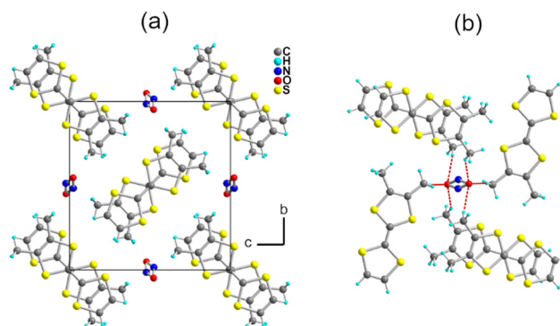
Fig. 2 (a) Projection view along a of the unit cell of ( o -DMTTF) _2\text{NO}_2 . (b) Details of the C-H \cdots O hydrogen bonds (red dotted lines).
