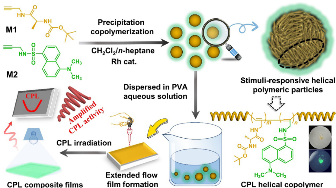
Scheme 1 Schematic illustration for constructing stimuli-responsive helical polymeric particles and composite films with amplified CPL.
