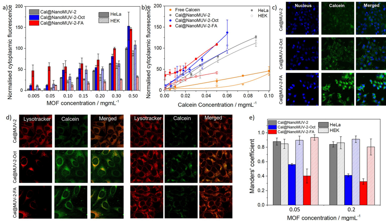
Fig. 5 (a) Endocytosis efficiency of calcein-loaded MOFs. Cytoplasmic fluorescence was normalized towards Cal@NanoMUV-2 at 0.5 mg mL -1 concentration for HeLa cells. (b) Endocytosis efficiency of functionalized NanoMUV-2 compared to uncoated NanoMUV-2 and free calcein. Cytoplasmic fluorescence was normalized towards the untreated controls (as a fold increase). Error bars represent the standard deviation of 3 independent experiments. (c) Confocal microscopy images of HeLa cells upon treatment with 0.2 mg mL -1 of calcein-loaded MOFs for 2 hours. (d) Confocal microscopy colocalization studies upon treatment with 0.05 mg mL -1 for 2 hours (right HeLa cells, left HEK cells). (e) Manders' correlation coefficients extracted from colocalization studies. Error bars correspond to the standard deviation of 5 independent images.
