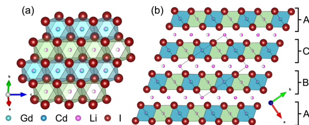
Fig. 7 (a) Mixed chain-like layer and (b) staggered stacking of the mixed chain-like and solely lithium containing layers in \text{Li}_{1.5+5x}\text{Cd}_{0.5-x}\text{Gd}_{0.5-x}\text{I}_4 with x = 0.14 . While the green octahedra are exclusively occupied with lithium, the blue octahedra in the mixed chain-like layers are occupied with lithium, gadolinium and cadmium.
