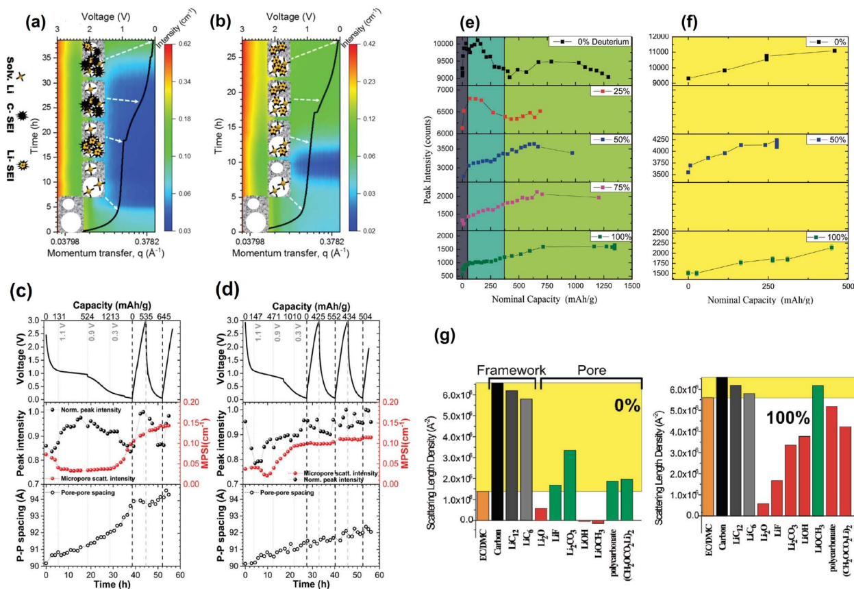
Fig. 16 SANS intensity (cm -1 ) as a function of the scattering vector q , 1st discharge time and voltage for (a) the 1 M LiTFSI/PC electrolyte system and (b) the 4 M LiTFSI/PC electrolyte system. Electrochemical and operando , and SANS analysis results for the 1 M (c) and (d) the 4 M electrolyte systems – (Top) electrochemical cycling profile; (middle): integrated Gaussian peak intensity for pore ordering and micropore (high q ) scattering intensity (MPSI); (bottom) pore–pore spacing determined by the Gaussian peak position. Reproduced with permission from ref. 86. Copyright © 2019, Royal Society of Chemistry. (e and f) Results of fits to in situ SANS data from the Gaussian peak corresponding to the pores in hard carbon with a LiPF 6 in EC:DMC electrolyte. The discharge process is given on the left and charge process on the right, while background colors indicate stages (I) (purple; initial discharge; 2.5–1.3 V), (II) (blue; SEI formation; 1.3–0.7 V), (III) (green; lithium intercalation; 0.7 V–5 mV), and (IV) (yellow; charging; 5 mV–3 V) of the initial charge/discharge cycle. (g) Plots comparing the calculated scattering length densities (SLDs) of the electrolytes, carbon framework, and potential components of the solid-electrolyte interphase (SEI) layer as a function of deuterium level. The deuterium level of the electrolytes varies from 0% to 100%, and the SLDs of the SEI layer have been adjusted accordingly for each case. The yellow band indicates the region over which a component in the SEI will result in a decrease in contrast between the framework and pore relative to a fresh cell, and these components have been highlighted in green for each deuterium level. Only the Li 2 O and LiOH components will cause an increase in contrast for all deuterium levels. Reproduced with permission from ref. 87. Copyright © 2012, American Chemical Society.
