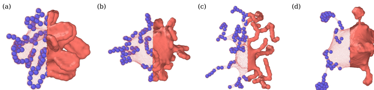
Fig. 8 Vesicle shapes for \phi = 0.04 and \epsilon = 3.5k_B T at (a) Pe = 15 (see Movie S4, ESI†), (b) Pe = 50 , (c) Pe = 150 (see Movie S1, ESI†), and (d) Pe = 300 . Particle structures change from membrane-wrapped ring-like arrangements to membrane-wrapped (branched) tubular aggregates, as Pe is increased. A further increase in Pe leads to the detachment of ABPs from the membrane and their accumulation at the tether end. The left half of the membrane is made transparent so that the arrangement of ABPs is visible.
