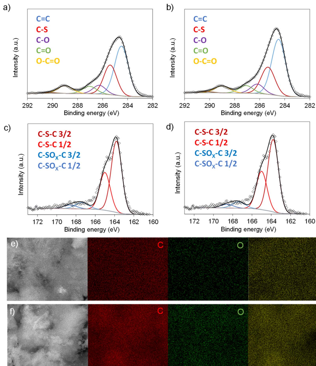
Fig. 1 High-resolution C 1s spectra of (a) AGS-600 and (b) AGS-750; high-resolution S 2p spectra of (c) AGS-600 and (d) AGS-750; EDX mappings of C, O and S for (e) AGS-600 and (f) AGS-750.
