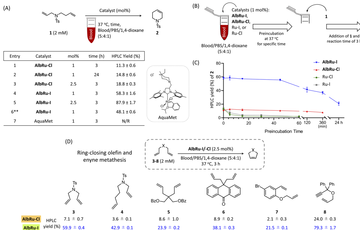
Fig. 2 Catalytic activity investigation of Ru-based ArMs for ring-closing metathesis in blood. (A) Reactivity studies of substrate 1 (2 mM) with AlbRu-Cl or I (1 or 2.5 mol%) and AquaMet catalyst (1 mol%) in a mixture of blood/PBS/1,4-dioxane (5 : 4 : 1) (**8 : 1 : 1). (B) To determine the time and extent of Ru protection, a series of experiments were run as illustrated. The indicated Ru catalysts (1 mol%) were preincubated in blood for a specific time (0, 5, 15, 30, and 60 min for Ru-I/Cl ; 0, 5, 15, 45, 120, and 360 min for AlbRu-Cl ; and 0, 5, 15, 45, 120, and 360 min, and 24 h for AlbRu-I ), followed by reaction initiation using 1 (2 mM). After a reaction time of 3 h, the yield of 2 was measured. (C) Graphical representation of stability results of the Ru catalysts in blood. (D) Substrate scope for testing ring-closing olefin and enyne metathesis. Given HPLC yields were determined by HPLC analysis (peak retention times relative to product standards, followed by MS analysis for confirmation, and calculation of resultant yields based on product standard curves). Error bars represent the s.d. of three independent measurements. The blood used here was commercially available sheep blood. Abbreviations: Ts, 4-toluenesulfonyl; N/R, no reaction.
